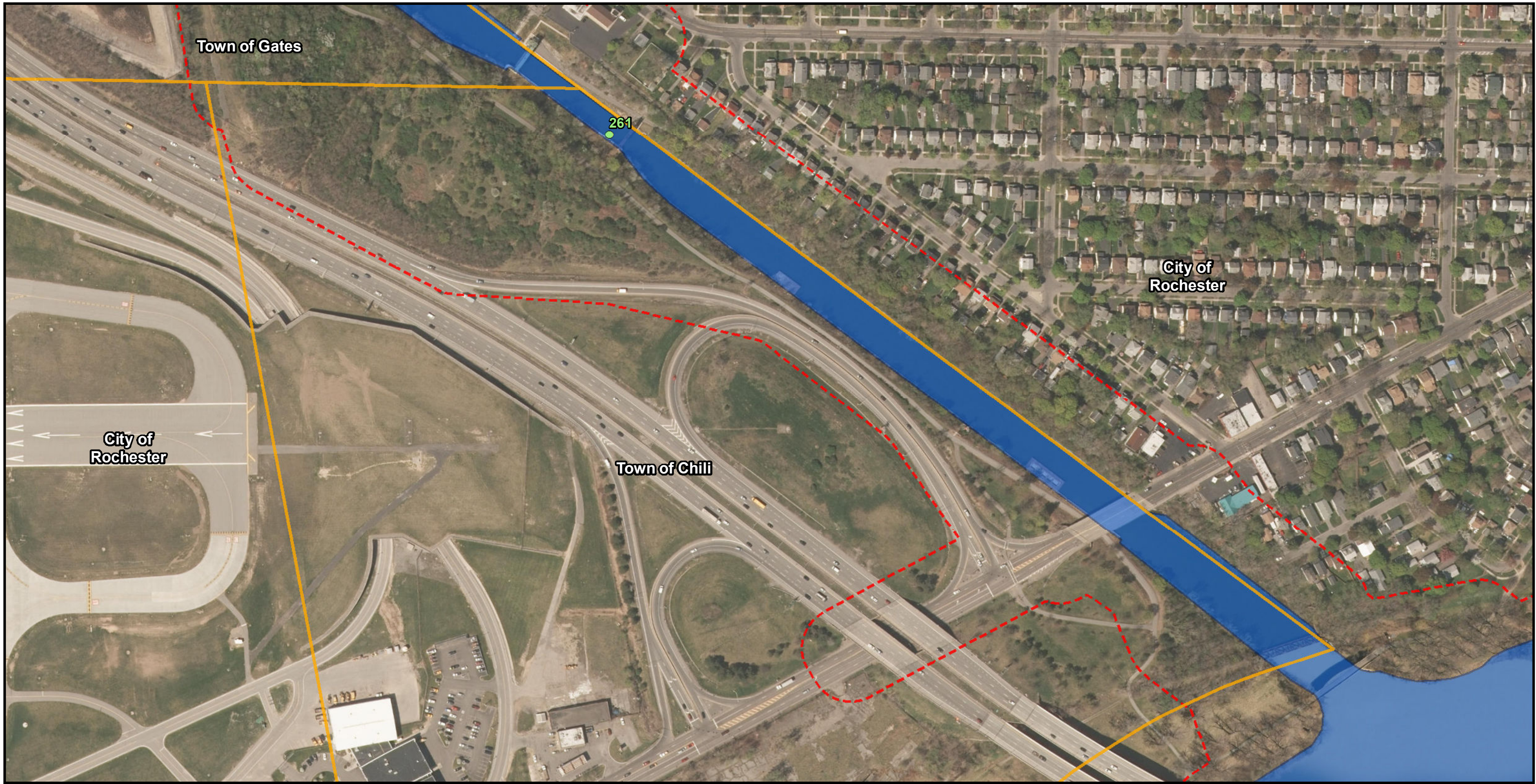
Figure 102F: Aquifers
